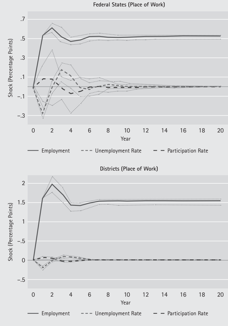
Figure 19: Adjustment of employment, unemployment and participation to a labour demand shock (Place of Work)
